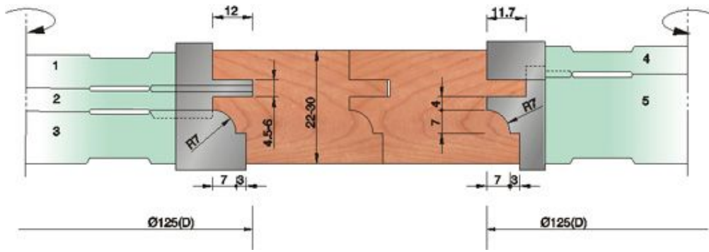
TF605BD125*d35*Z4 1SET/5PCS
