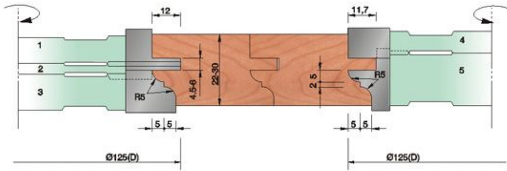
TF605CD125*d35*Z4 1SET/5PCS
