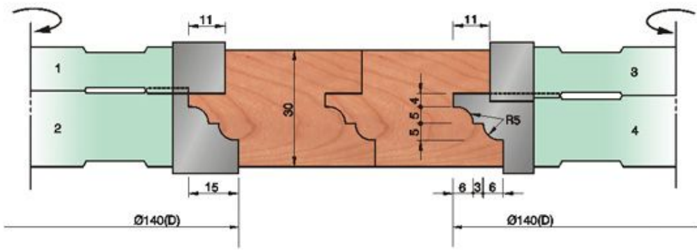
TF607ED140*d35*Z4 1SET/4PCS
