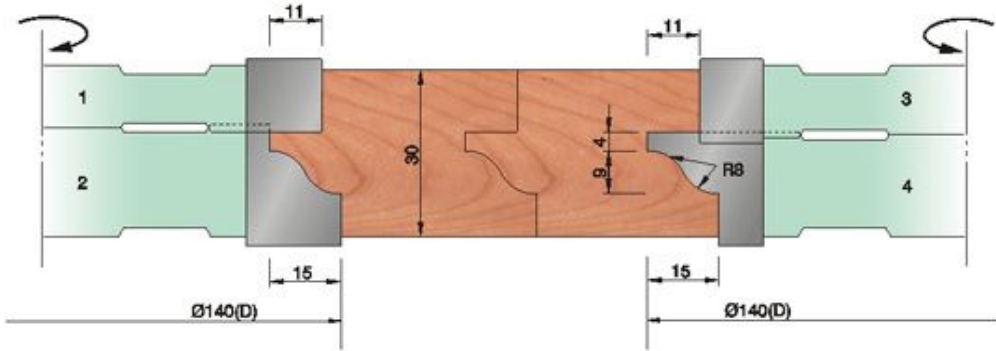
TF607FD140*d35*Z4 1SET/4PCS
