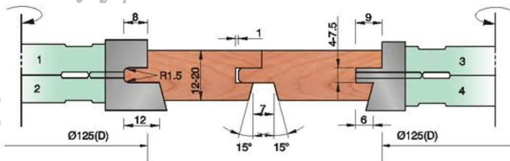
TF601QD125*d40*Z4/Z6 1SET/4PCS
