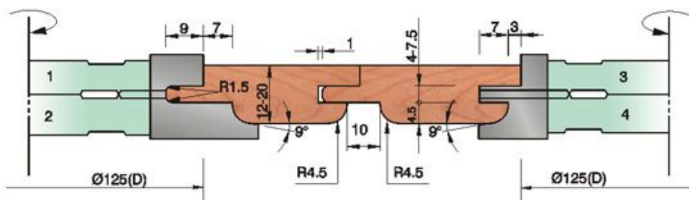
TF601QD125*d40*Z4/Z6 1SET/4PCS
